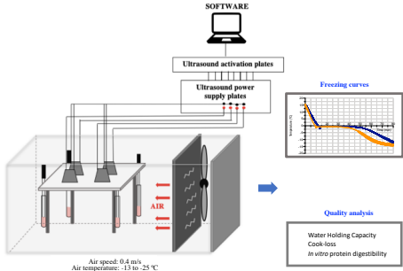
Freezing air-forced tunnel
