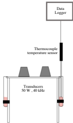
Direct contact US system
